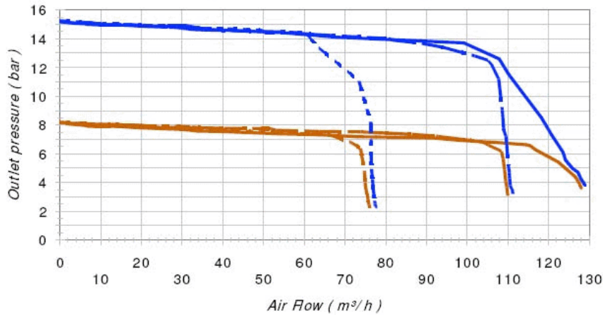
REGULATOR FLOW CURVE 896 15 bar
