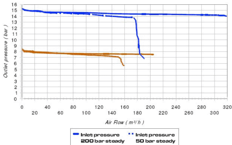
REGULATOR FLOW CURVE 825 15 bar
