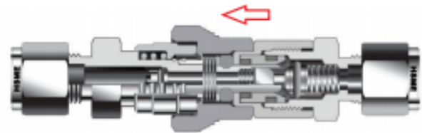
Double-End Shutoff (DES) Shutoff Stem Coupled with Standard Shutoff Body
