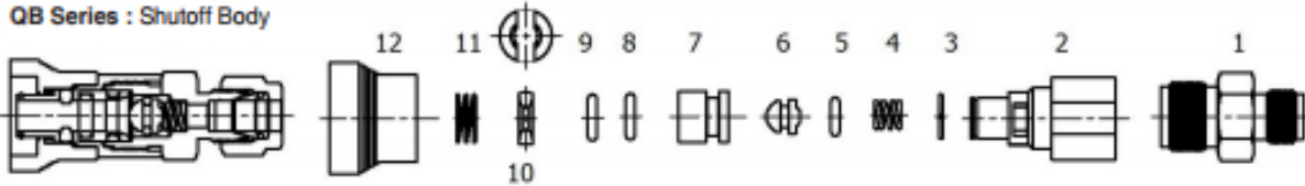
Single-End Shutoff (SES) No Shutoff Stem Coupled with Standard Shutoff Body
