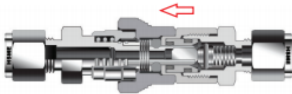
Single-End Shutoff (SES) No Shutoff Stem Coupled with Standard Shutoff Body
