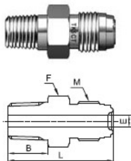
Male Connector (NPT)
