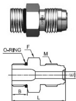
Male Connector (ST)
